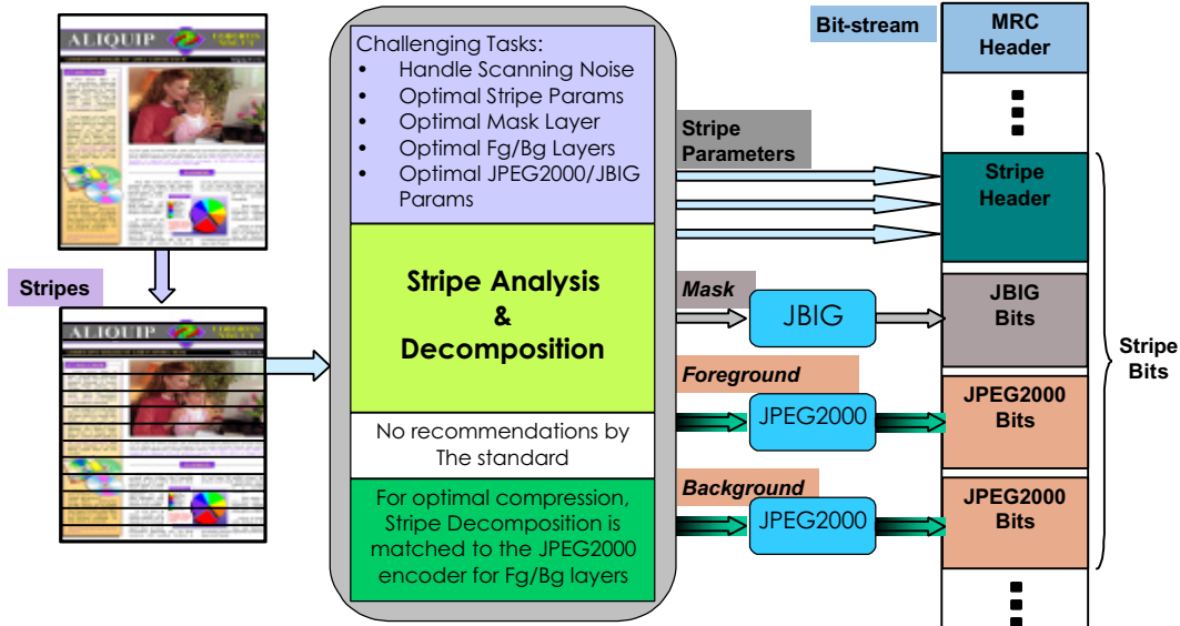
Figure 1. Schematic of the MRC encoder
